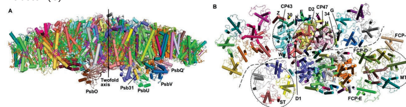
Figure 3. Cryo-EM structure of the PSII-FCP supercomplex from a diatom viewed from the side of the membrane (A) and top of the stromal side (B).
