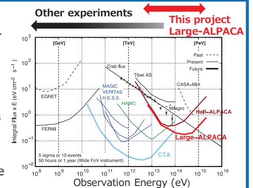
Figure 2. Sensitivity to gamma-ray intensity of cosmic gamma-ray observatories in the world as a function of observation energy.
