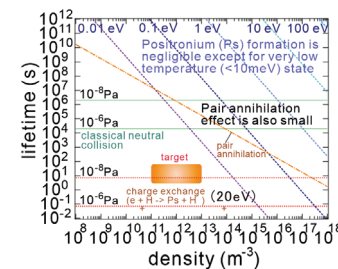
Figure 3. Positron life times
