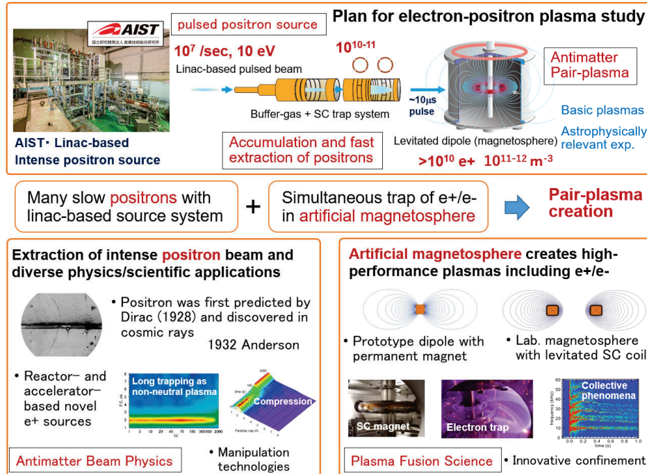
Figure 1. Electron-positron plasma investigation with pulsed positron source and levitated dipole
