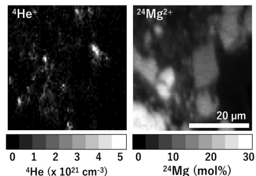
Figure 1. Two-dimensional distribution of solar wind He (left) and mineral particles (right) in matrix of gas-rich chondrite NWA 801.
