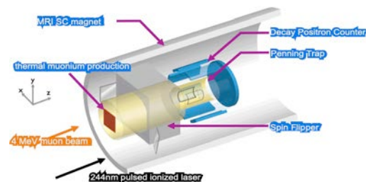
Figure 1 Concept of Muon Trap
