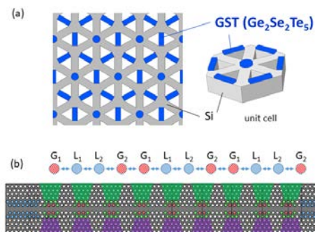
Figure 1 Reconfigurable topological nanophotonics structures. (a) GST tuning, (b) Non-Hermitian tuning.
