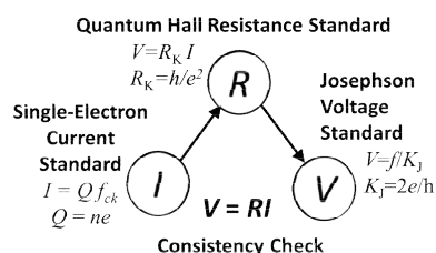
Fig. 1 Quantum metrology triangle (QMT)
