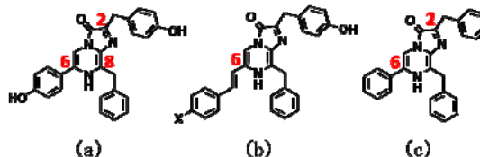
図1 (a)CTZ (b)6-pi-X-CTZ (c)DeepBlueC™
