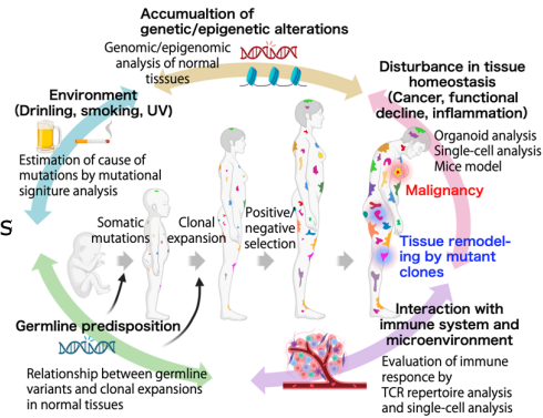
Fig.1 Research concept
