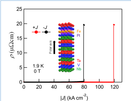
Figure 2. Nonvolatile superconducting diode
