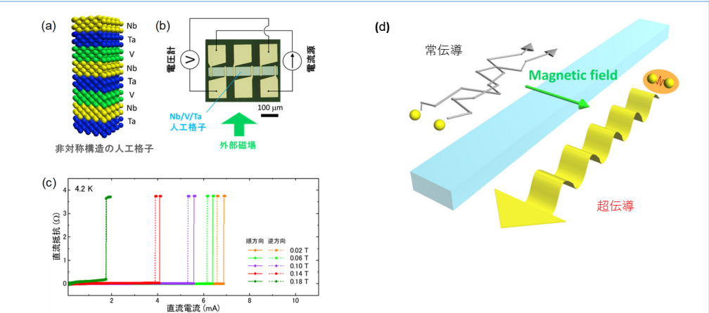
Figure 1. Superconducting diode effect
