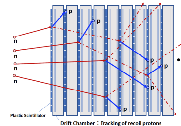
Figure 3. Schematic Figure of our new neutron detector array
