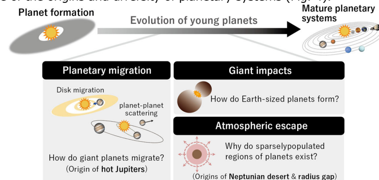
Figure 4. A conceptual diagram of what we are aiming to reveal in this study.
