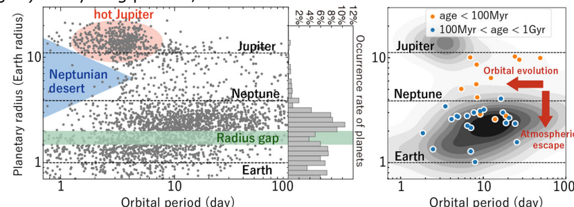
Figure 3. The periods and radii for known transiting planets: The left side represents the distribution for planets aged over 1 Gyr, while the right side compares planets less than 1 Gyr with the older population contour. Young planets are believed to evolve significantly within their first 1 Gyr. This evolution involves orbital migration toward the inner regions and atmospheric escape leading to reduced radius and mass.
