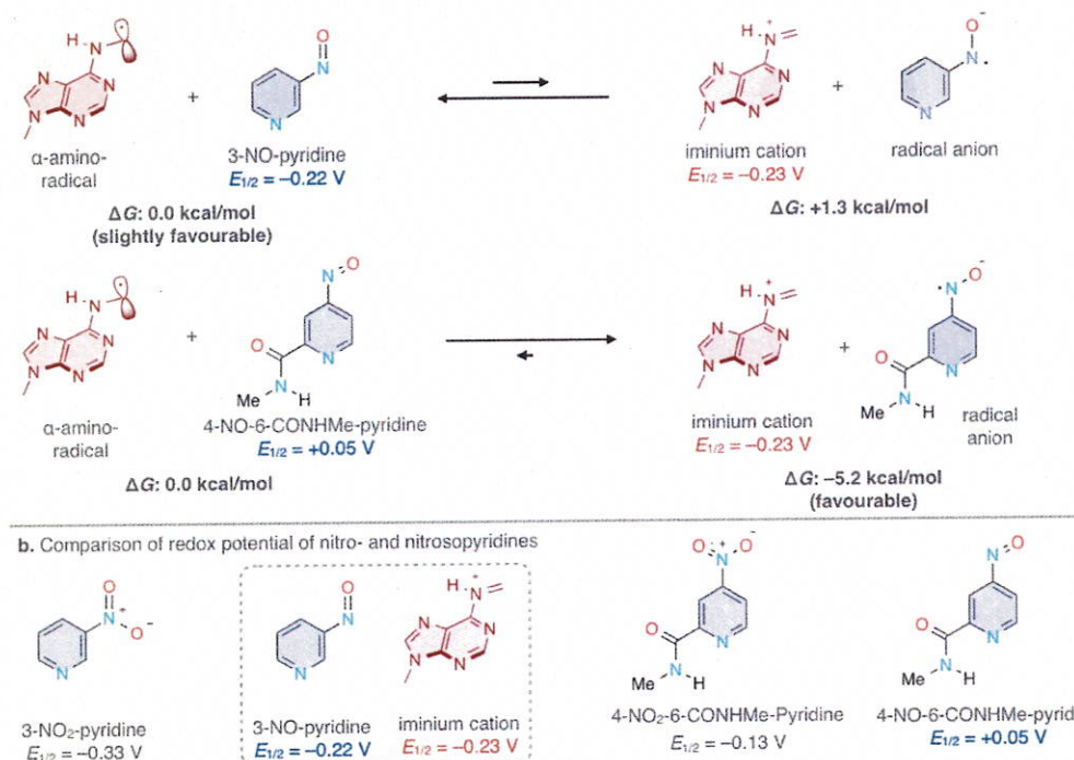
Figure 2-4. a. Energetic analysis of SET between \alpha -amino radical and nitroso compounds at Redox potentials of nitro-pyridine derivatives and Adenine at CAM-B3LYP-D3(BJ)/6-311++(2df,2p)/SMD(water)//CAM-B3LYP/6-31+(d,p) 298K level of theory. b. redox potential: CAM-B3LYP/6-31+G(d,p)/SMD (water) at 298 K level of theory;
