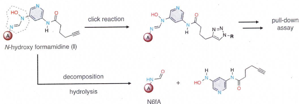
Figure 3-1. Derivatization of modified adenine bearing a N -hydroxy formamidine structure and degradation via hydrolysis.
