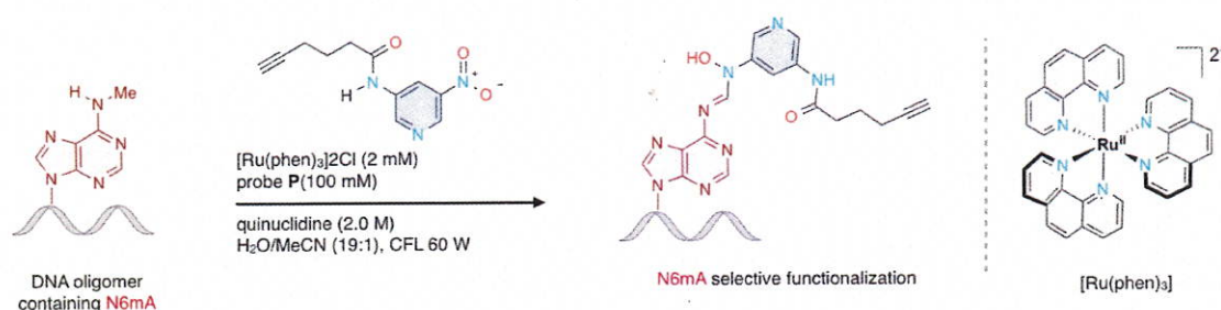
Figure 1. Proposed reaction pathway for N-methyl selective functionalization of adenine (N6mA).
