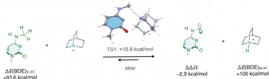
b. HAT between N4mC and quinuclidine radical cation
