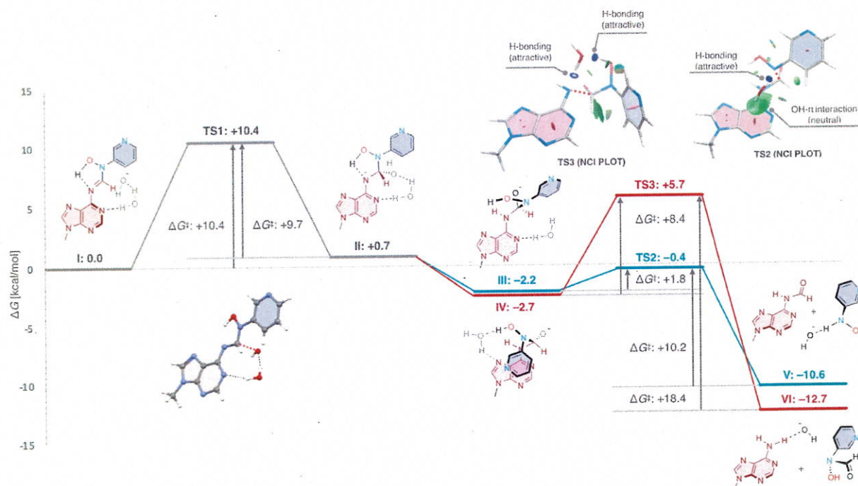
Figure 3-2. Energetic analysis of hydrolysis pathway of N -hydroxy formamidine I at B3LYP-D3(BJ)/6-311++(2df,2p)/SMD(water)//B3LYP-D3(BJ)/6-311+(d,p)/SMD(water) 298K level of theory.
