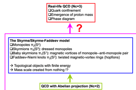
Fig.3.5. Particle/nuclear physics fundamental insights arising from fusing topology & chirality paradigms by the SKCM 2 Center.
