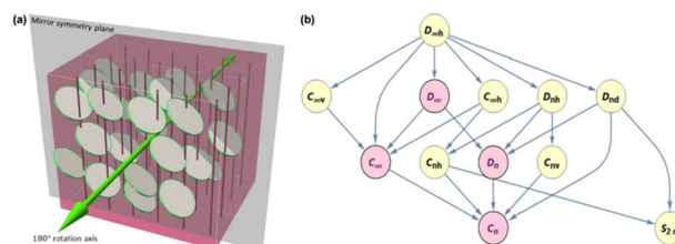
Fig.3.6. Molecular-colloidal nematic LCs. (a) Monoclinic nematic formed by thin discs dispersed in a nematic host with molecular ordering direction shown by magenta lines. The symmetry plane & axis are marked. Green regions next to particle edges are regions where order of the molecular host is perturbed by the colloidal surfaces. (b) Point group symmetries & transformations of orientational order that can emerge in mesostructured nematic LCs formed by a uniaxial D_{\infty h} molecular host doped with colloidal particles with various geometric shapes. Chiral & nonchiral phases are depicted with magenta & yellow colors, respectively.
