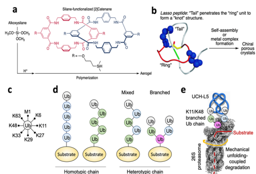
Fig. 3.10. Chemical design strategies of knotted molecular crystals & gels based on (a) silane-functionalized catenanes & (b) proteins, & the naturally occurring (d-e) protein knotting in biological systems.
