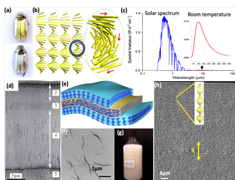
Fig. 3.9. Natural & bioinspired helicoidal structures & solitons. (a) Photos of Chrysina resplendens , the gold scarab beetle (top), and Chrysina chrysargyrea , the silver scarab beetle (bottom), both achieving broadband optical reflections by helical structures in their cuticles. (b) Schematic of a chiral structure formed by cellulose nanocrystals mimicking that in cuticles. (c) Solar spectrum at Earth's surface & (inset) thermal spectrum at room T. (d) A cross-section through the outer part of the cuticle of Chrysina resplendens , showing regions: epicuticle (1) & exocuticle comprising upper helicoid (2) nematic-like layer (3) & lower helicoid (4), & endocuticle (5). Image from [J. Roy. Soc. Interface 14, 20170129 (2017)]. (e) Schematic of assembly with near-100% reflectivity formed by 2 helical layers separated by a nematic retarder, found in the cuticle. (f,g) A TEM image (e) of nanocellulose & a photograph of an aqueous colloidal nanocellulose at ~10 wt.% (g). (h) SEM image of the helical structure of cellulose nanocrystals.
