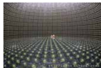
Inside of Super-Kamiokande
