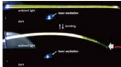
Optical waveguide
